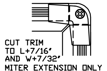
ALTERNATE CORNER DETAIL
