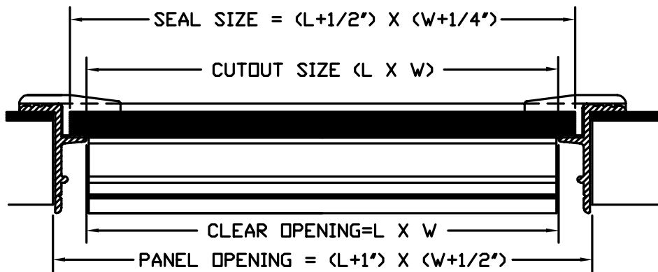
SECTION THROUGH CUTOUT
