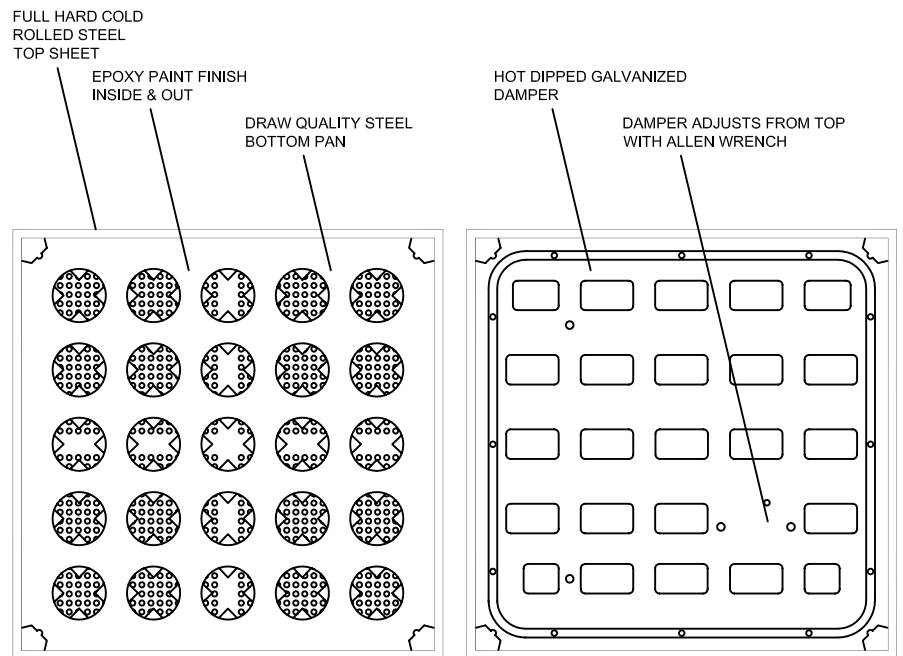
BOTTOM VIEW
