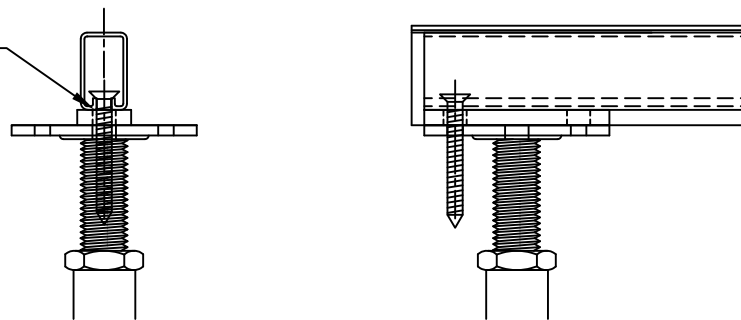
OPTIONAL ATTACHMENT METHOD FOR CUT STRINGER
